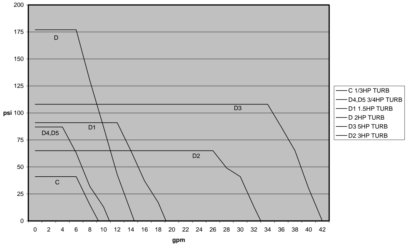
Turbine Pump Performance
